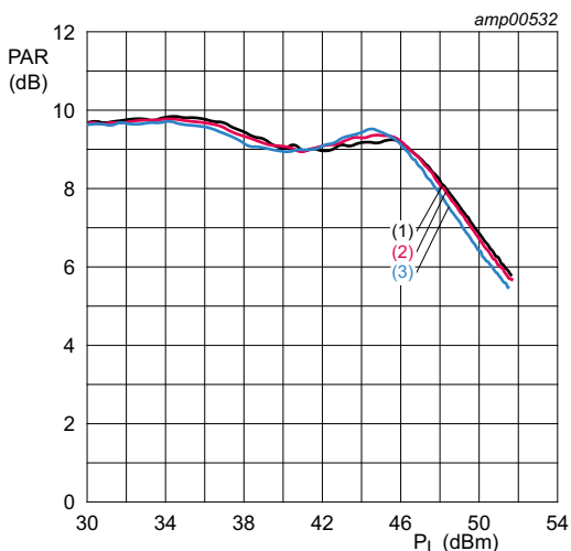
V_{DS} = 50\text{ V}; I_{Dq} = 380\text{ mA}; V_{GS(amp)peak} = 0.55\text{ V}. (1) f = 869\text{ MHz} (2) f = 881\text{ MHz} (3) f = 894\text{ MHz}
