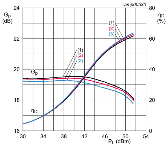
V_{DS} = 50\text{ V}; I_{Dq} = 380\text{ mA}; V_{GS(amp)peak} = 0.55\text{ V}. (1) f = 869\text{ MHz} (2) f = 881\text{ MHz} (3) f = 894\text{ MHz}
