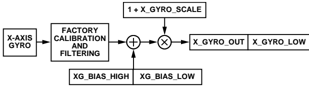
Figure 27. User Calibration Signal Path, Gyroscopes
